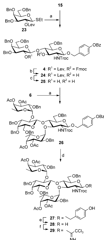
Scheme 3. Synthesis of the Le y donor. a) NIS, TESOTf, \text{CH}_2\text{Cl}_2 , 0^\circ\text{C} ; b) \text{CH}_2\text{Cl}_2/\text{Et}_3\text{N} 5:1, 95%; c) \text{NH}_2\text{NH}_2\cdot\text{HOAc} , MeOH, \text{CH}_2\text{Cl}_2 , 87%; d) \text{H}_2\text{O}_2 , \text{Et}_3\text{N} , THF, 82%; e) DDQ, \text{CH}_2\text{Cl}_2/\text{H}_2\text{O} 95:5, 78%; f) \text{CCl}_3\text{CN} , DBU, \text{CH}_2\text{Cl}_2 , 91%.
