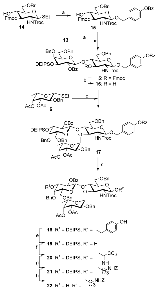
Scheme 2. Synthesis of the Le x acceptor. a) p -(benzoyl)-benzyl alcohol, NIS, TESOTf, CH 2 Cl 2 , 0°C, 86%; b) CH 2 Cl 2 /Et 3 N 5:1, 95%; c) NIS, TESOTf, CH 2 Cl 2 , 0°C, 74%; d) H 2 O 2 , Et 3 N, THF, 80%; e) DDQ, CH 2 Cl 2 /H 2 O 95:5, 81%; f) CCl 3 CN, DBU, CH 2 Cl 2 , 90%; g) BF 3 ·Et 2 O, CH 2 Cl 2 , 86%; h) TBAF, HOAc, THF, 82%.
