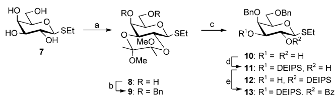
Scheme 1. Synthesis of galactose donor 13 . a) Butane-2,3-dione, HC(CH 3 ) 3 , CSA, MeOH, reflux, 78%; b) NaH, BnBr, DMF, 85%; c) TFA/H 2 O 9:1, 67%; d) DEIPSCl, imidazole, THF, 78%; e) BzCl, TEA, DMAP, CH 2 Cl 2 , 89%.
